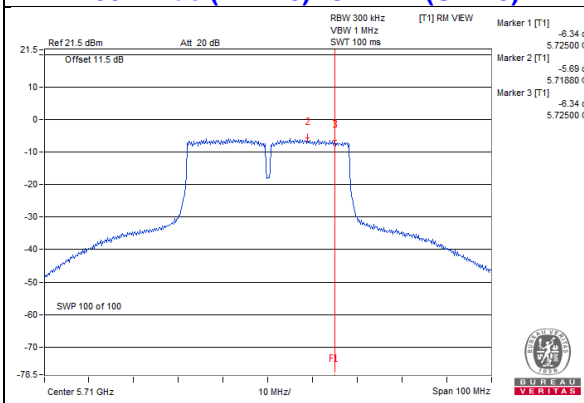
802.11ac (VHT40): CH 142 (UNII-3)
