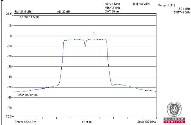
802.11ac (VHT40) / Chain 3 - CH110
