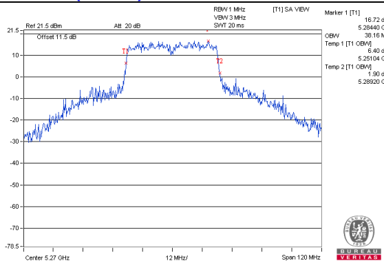
802.11ac(VHT40) / CH54
