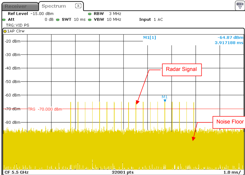
Radar Signal 3
