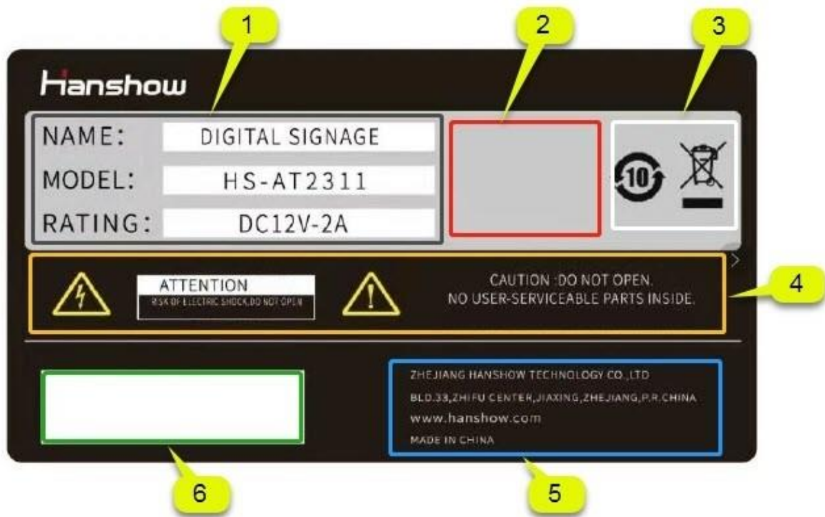
Figure 2-2 HS-AT2311 nameplate
