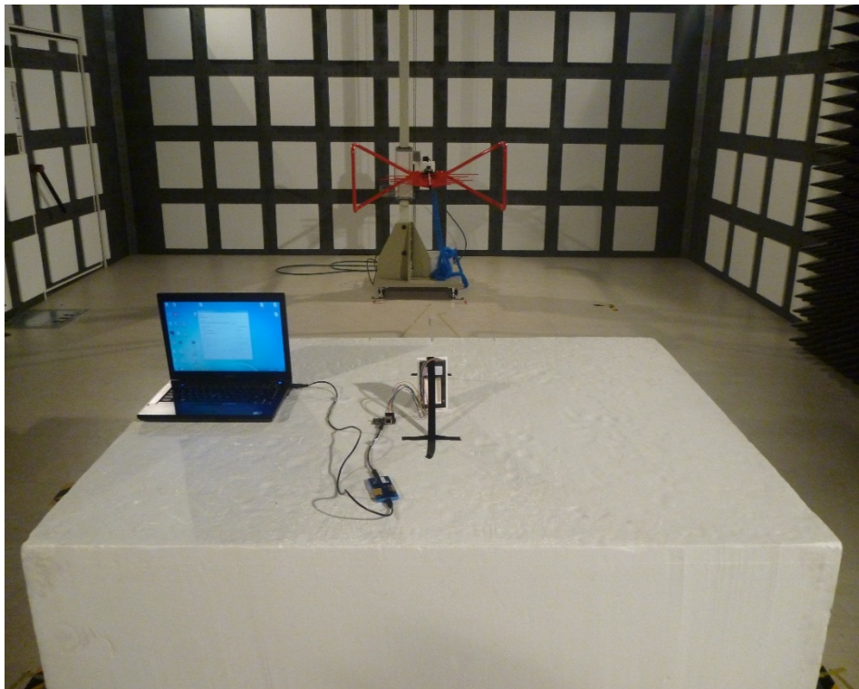
Radiated Emission -Rear View (Below 1GHz) Remote
