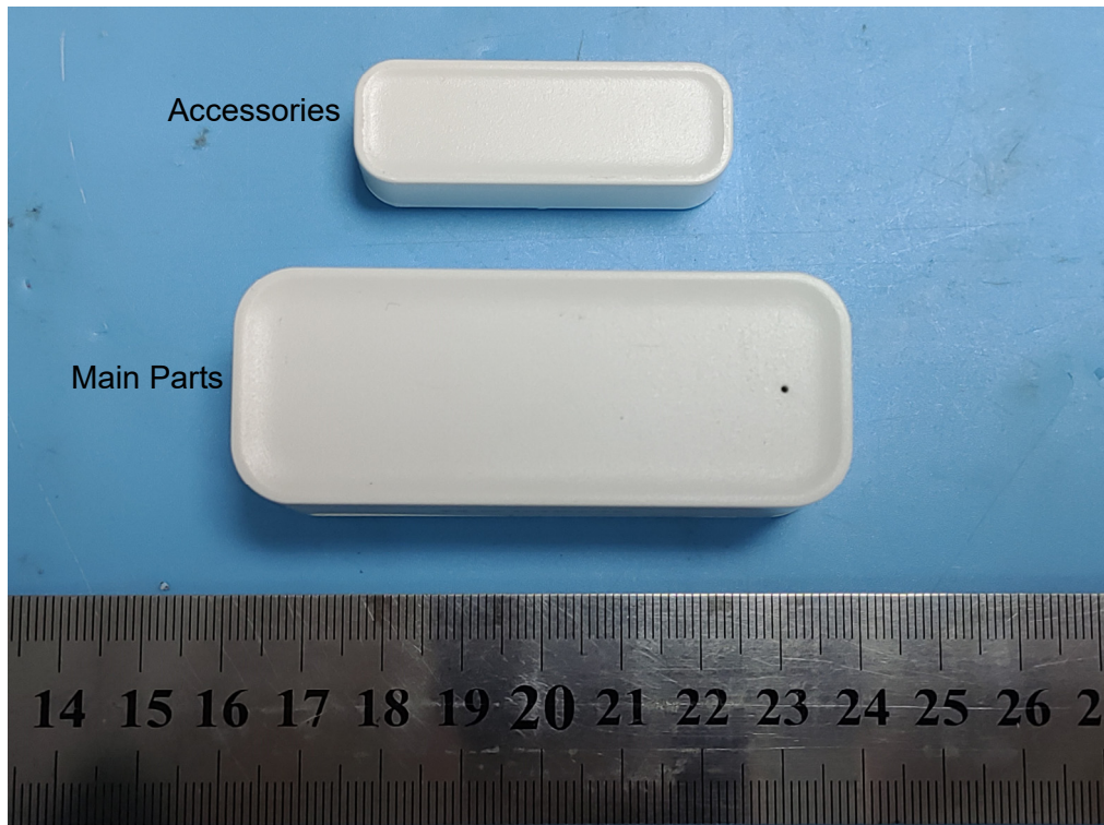
Main Parts
