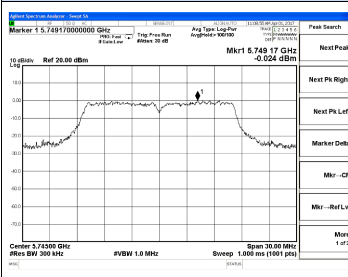
802.11a-5745MHz
