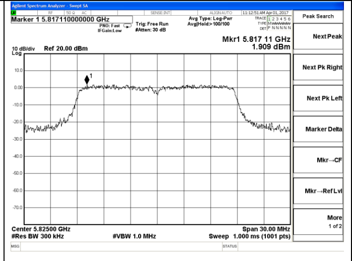
802.11n20-5825MHz
