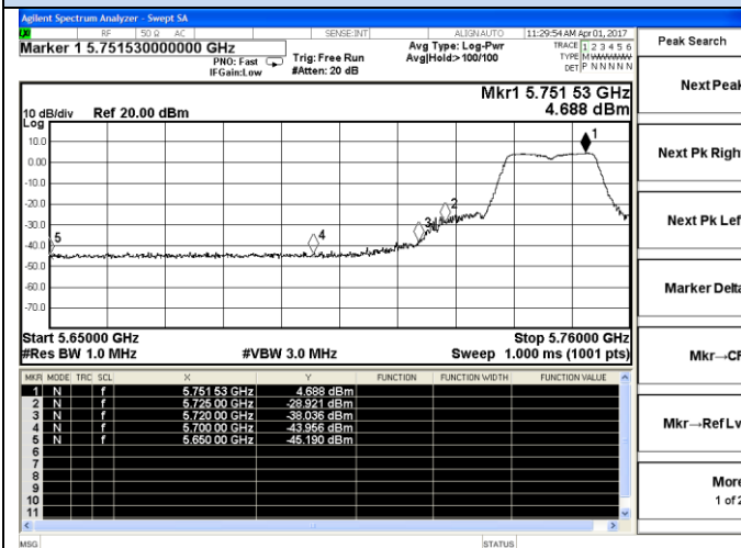
802.11n20-5745MHz-Lower
