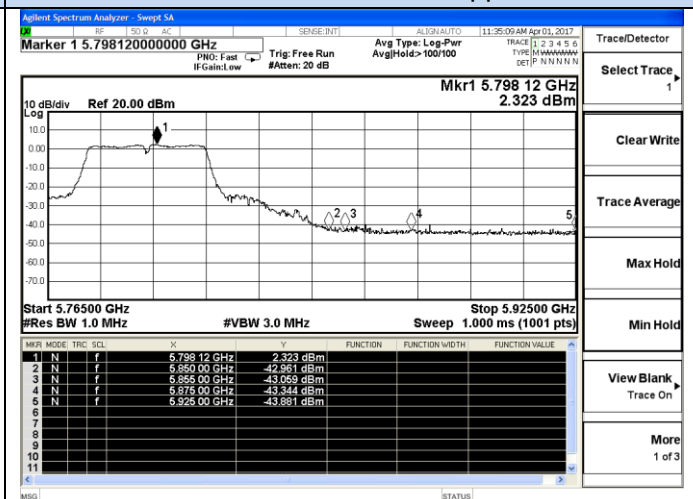
802.11n40-5795MHz-Upper
