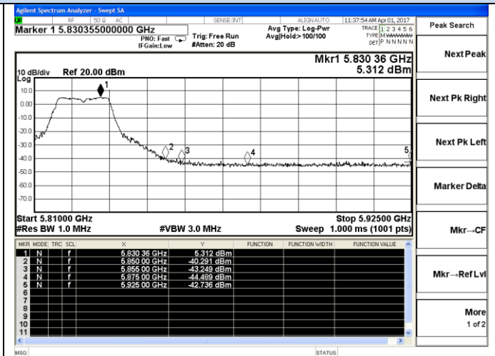
802.11a-5825MHz-Upper
