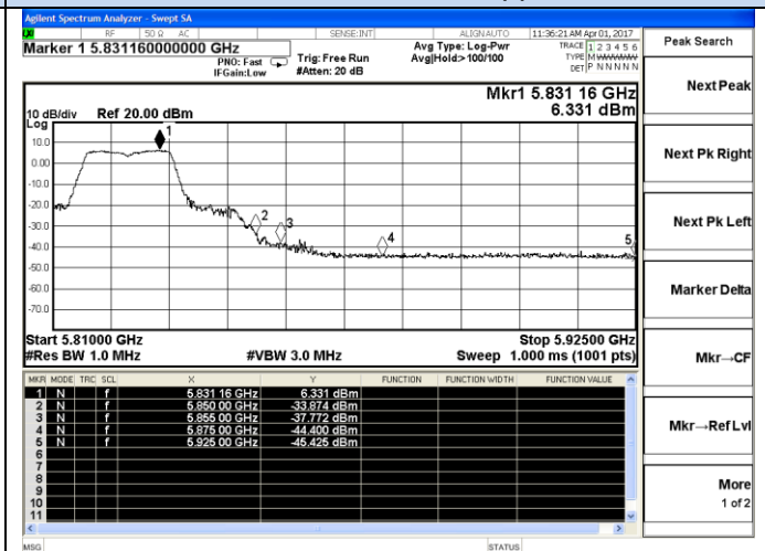
802.11n20-5825MHz-Upper
