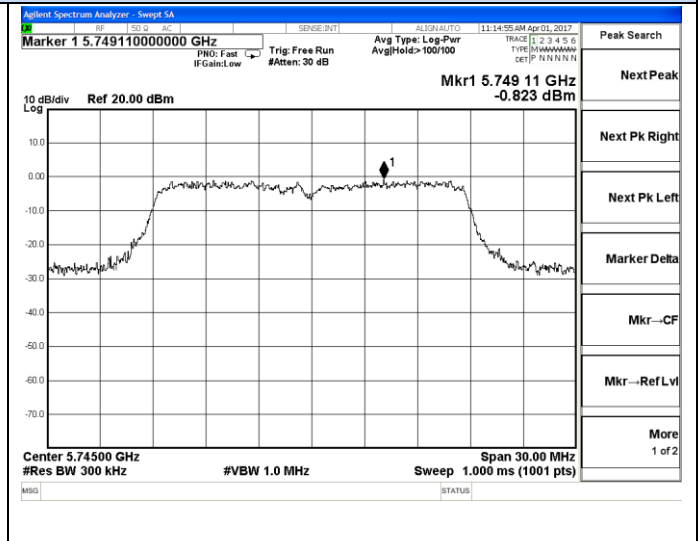
802.11n20-5745MHz
