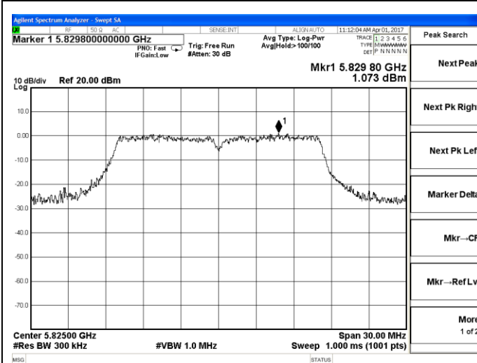
802.11a-5825MHz
