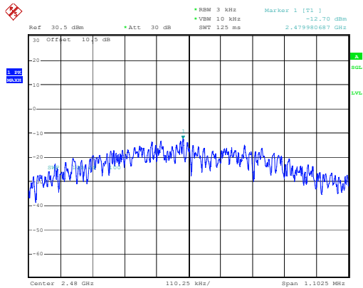
High Channel -12.70dBm/3kHz
