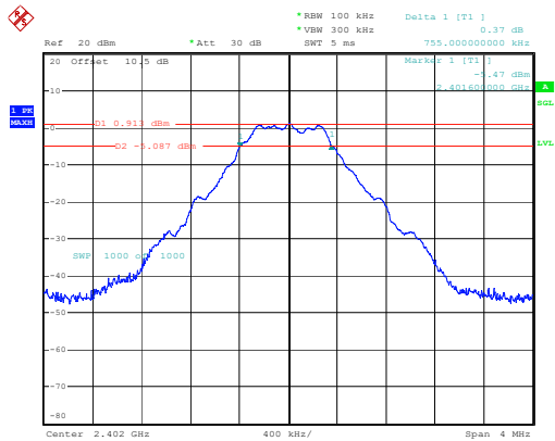
Low Channel 0.755MHz
