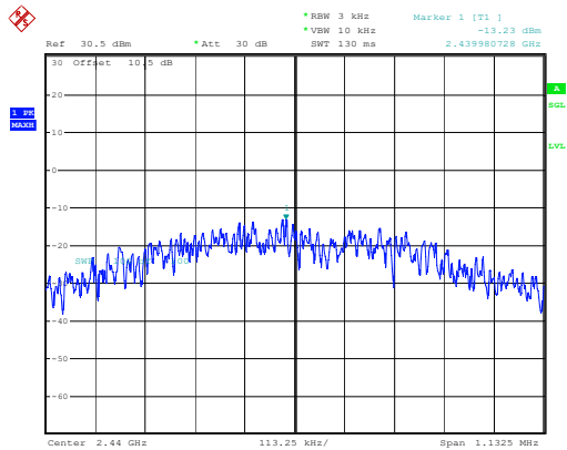
Middle Channel -13.23dBm/3kHz
