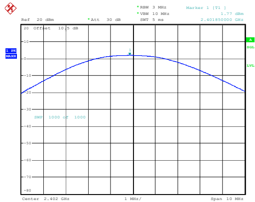
Low Channel 1.77dBm
