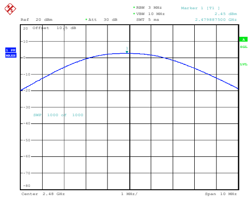
High Channel 2.45dBm
