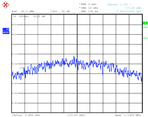
Low Channel -13.66dBm/3kHz
