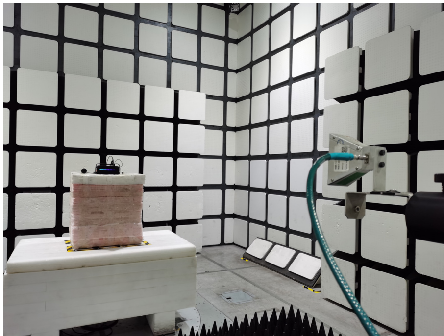
Radiated Emissions View (18-25 GHz)
