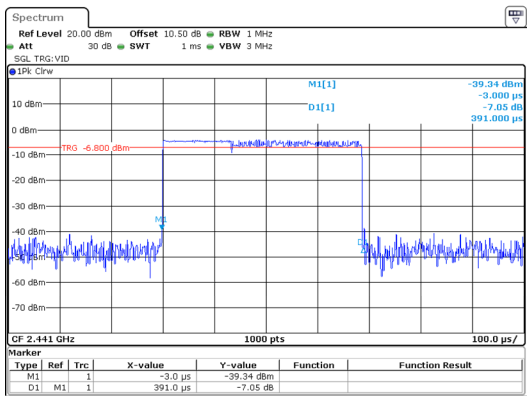
\pi/4 -DQPSK_Hopping_2DH1 0.391ms
