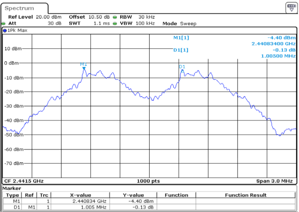
GFSK_Middle 1.005MHz
