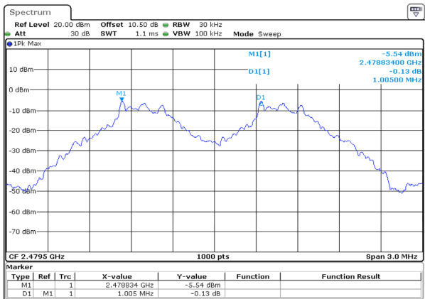
GFSK_High 1.005MHz
