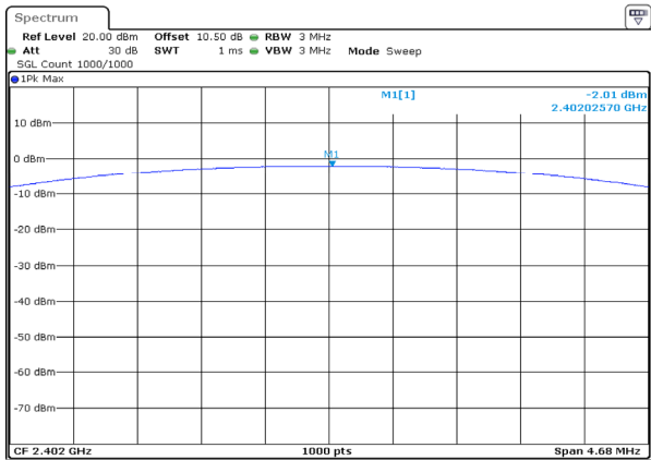
GFSK_Low -2.01dBm
