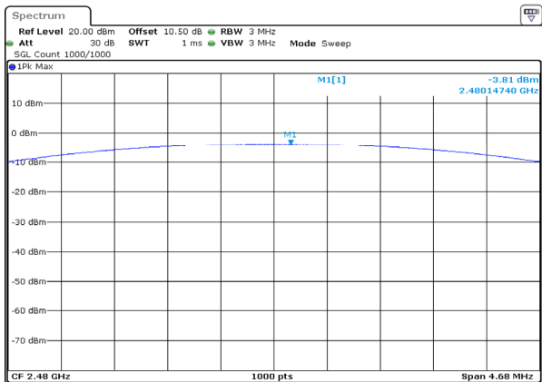
GFSK_High -3.81dBm
