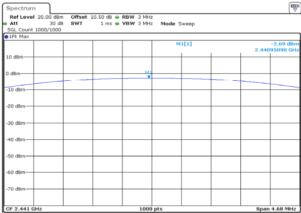
GFSK_Middle -2.69dBm
