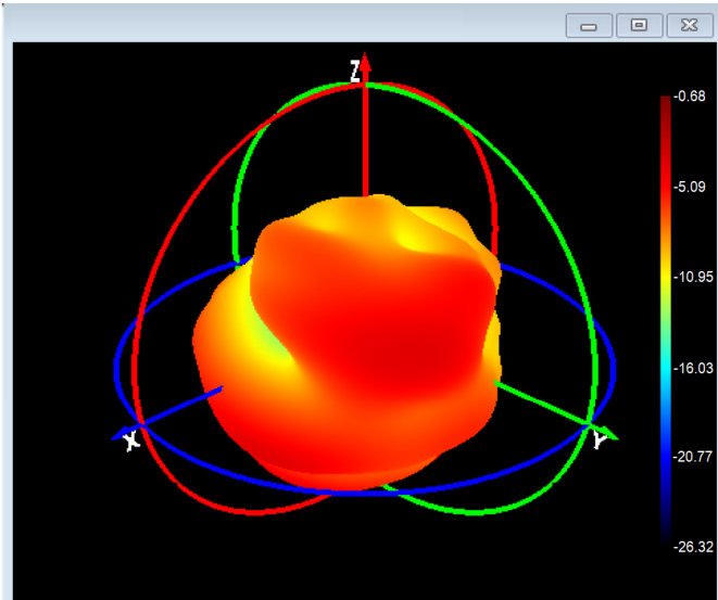
3D Radiation Pattern @ 2440 MHz
