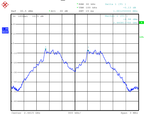
GFSK_Middle 1.001MHz
