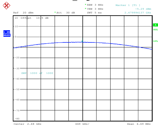
GFSK_High -5.29dBm
