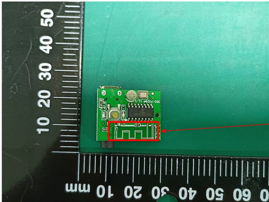
BT Antenna
