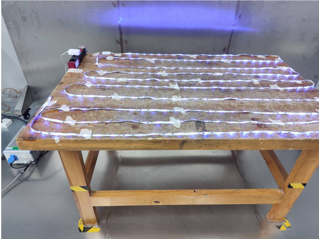
Conducted Emissions Side View(For model MLW7-1003-ICM)
