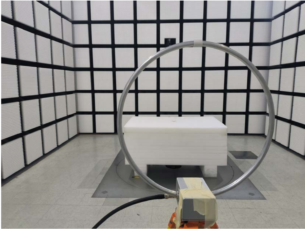
Radiated Emission Below 1GHz View Perpendicular
