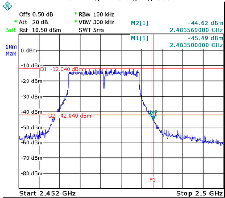
ANT0 TX 11g: Band edge-right side
