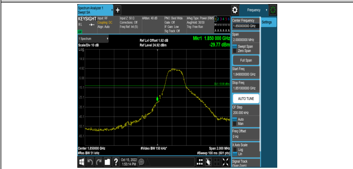
Band2-3MHz-16QAM-18615-1RB#14
