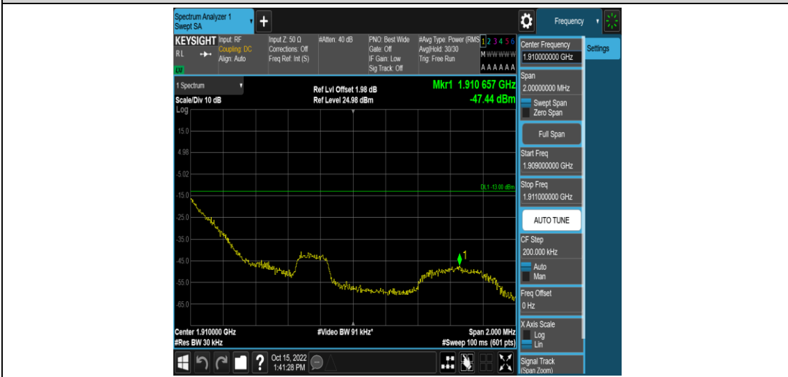
Band2-1.4MHz-16QAM-19193-1RB#5
