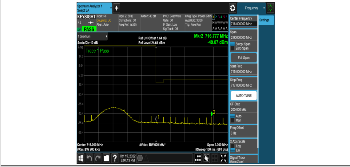
Band12-10MHz-QPSK-23130-1RB#49
