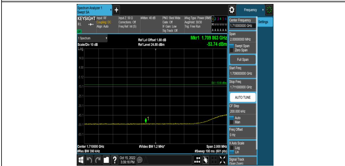
Band4-20MHz-16QAM-20050-100RB#0
