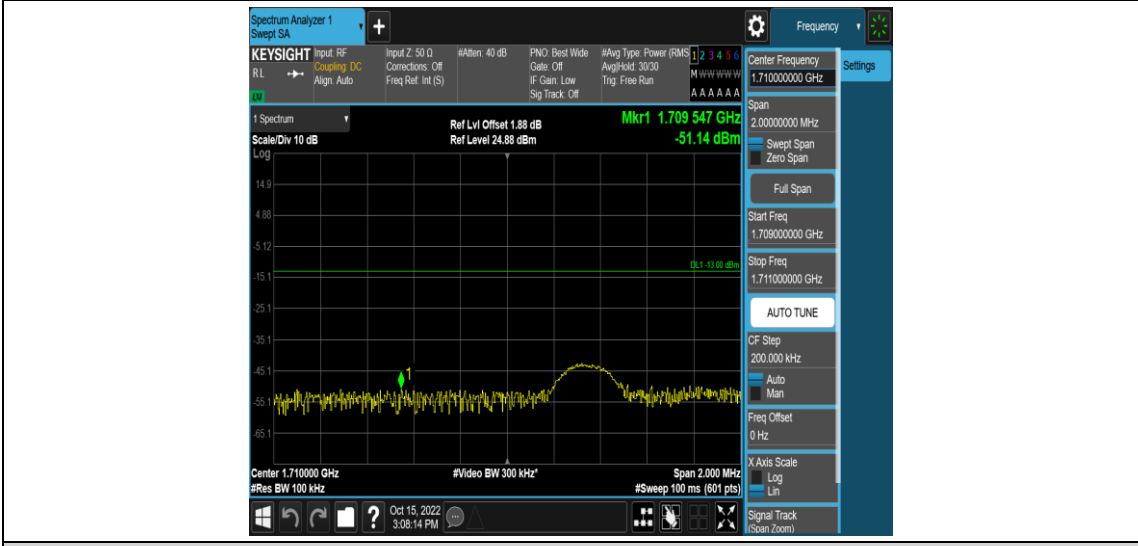
Band4-5MHz-16QAM-19975-25RB#0
