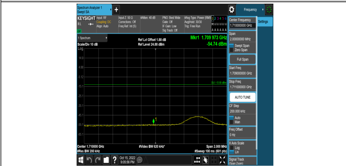
Band66-10MHz-16QAM-132022-50RB#0
