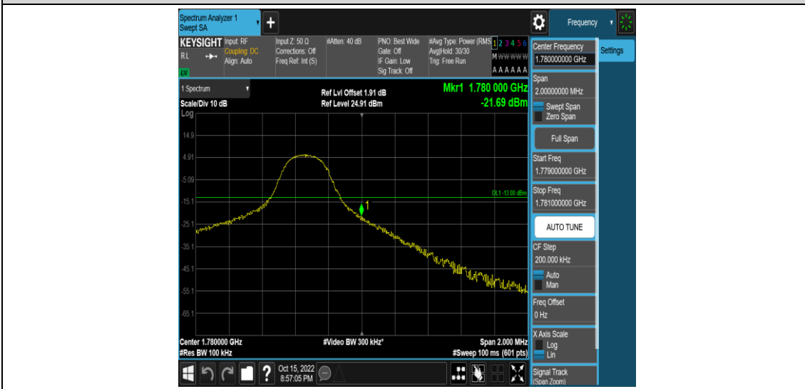
Band66-5MHz-QPSK-132647-25RB#0
