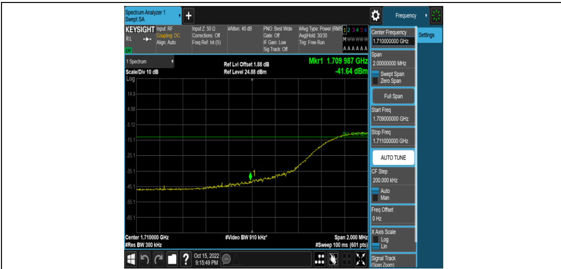
Band66-15MHz-16QAM-132597-1RB#0
