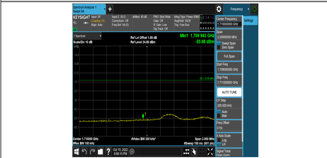
Band66-5MHz-16QAM-131997-25RB#0
