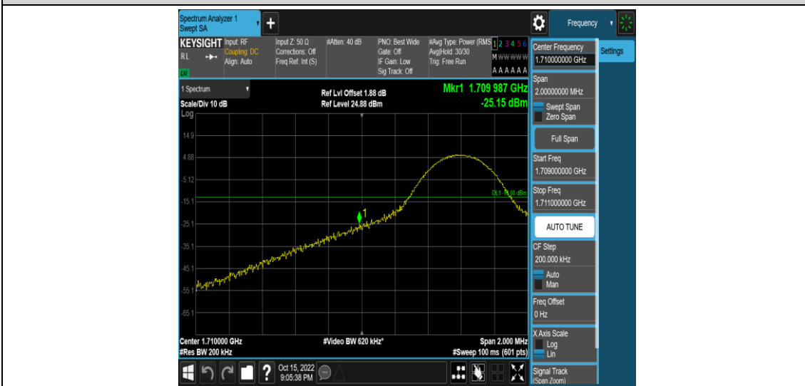
Band66-10MHz-16QAM-132022-1RB#49
