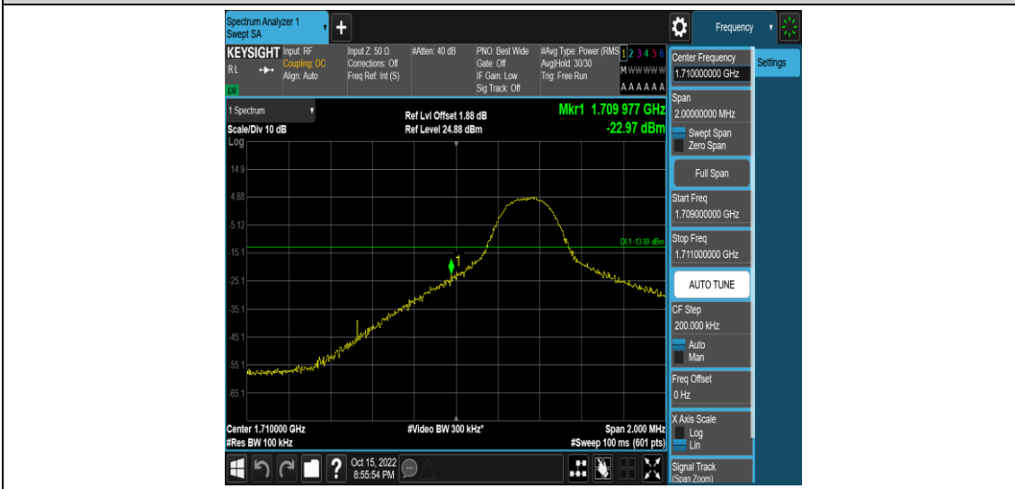
Band66-5MHz-16QAM-131997-1RB#24
