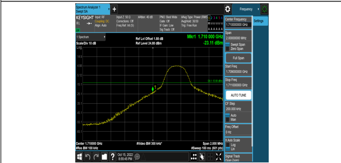
Band66-5MHz-QPSK-131997-1RB#24
