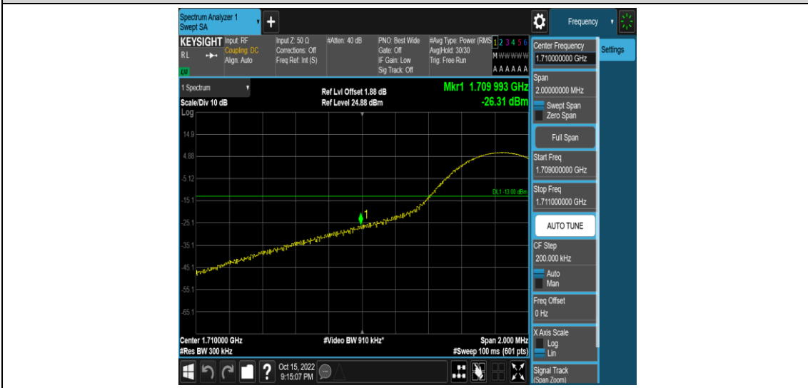
Band66-15MHz-QPSK-132047-1RB#74
