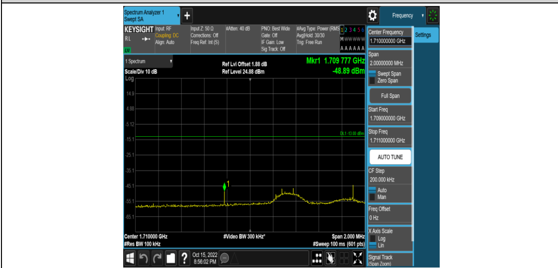
Band66-5MHz-QPSK-131997-25RB#0
