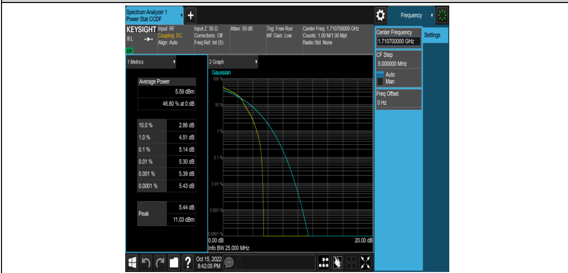
Band66-1.4MHz-16QAM-131979-6RB#0
