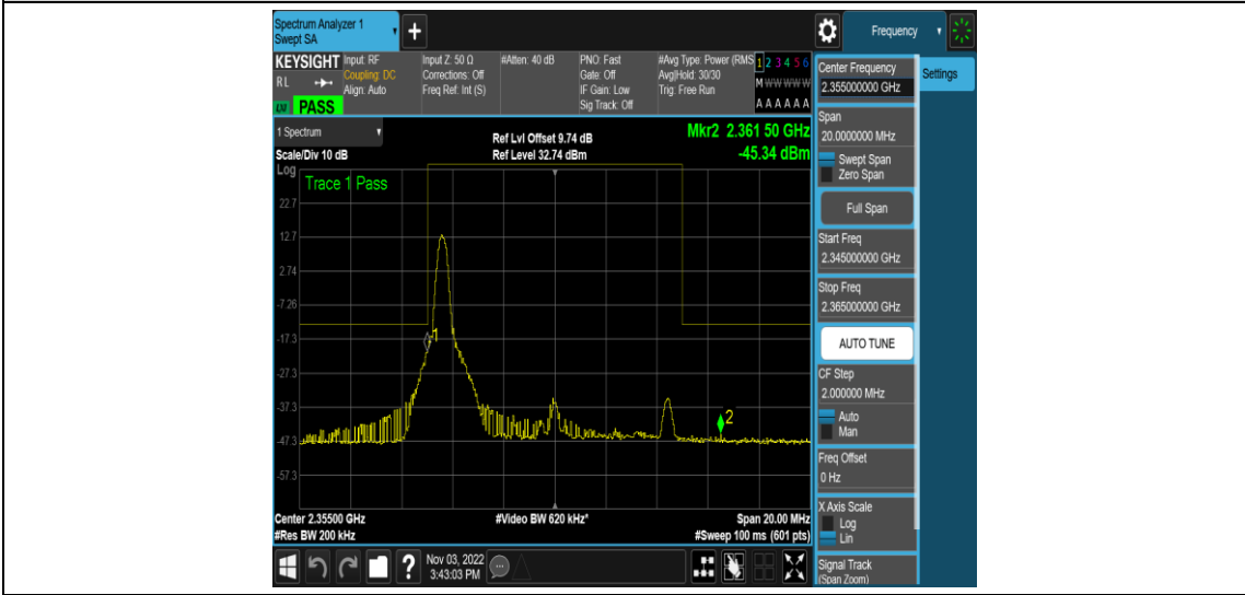
Band40-10MHz-16QAM-39200-1RB#49
