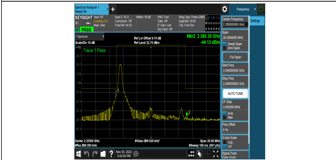
Band40-10MHz-QPSK-39200-1RB#49
