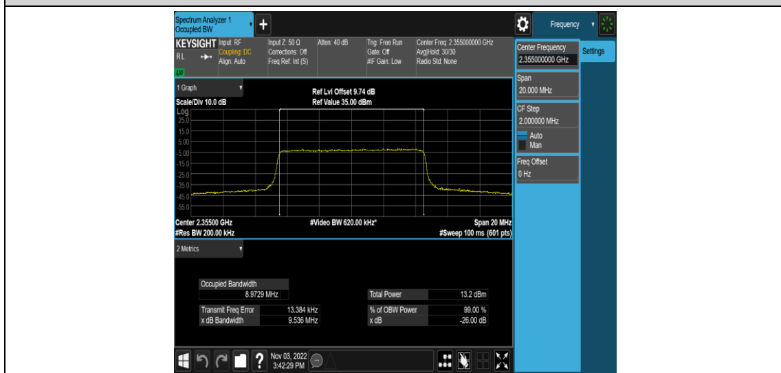
Band40-10MHz-16QAM-39200-50RB#0
