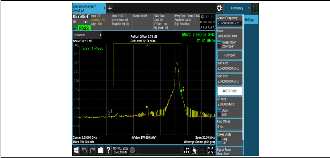
Band40-10MHz-16QAM-39200-50RB#0
