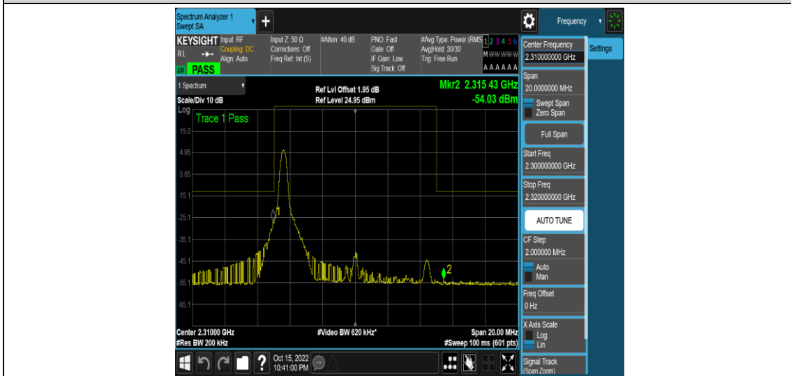
Band40-10MHz-QPSK-38750-1RB#49
