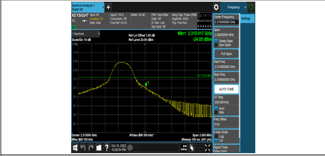
Band40-5MHz-16QAM-38775-25RB#0
