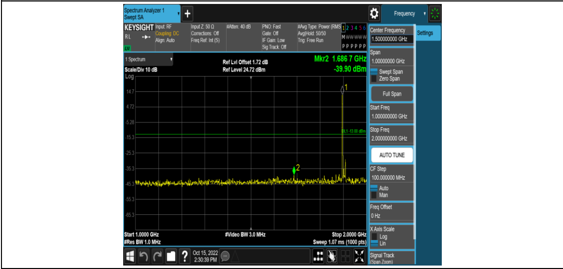
Band2-15MHz-QPSK-19125-1RB#0-Range5:2000~20000MHz
