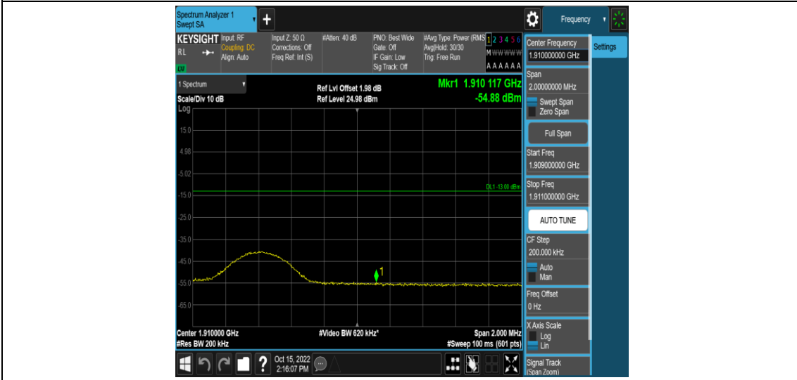
Band2-10MHz-16QAM-19150-1RB#49
