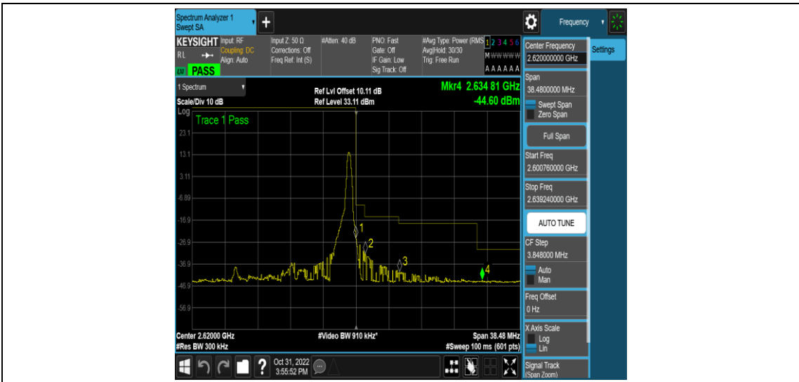
Band38-15MHz-QPSK-38175-75RB#0
