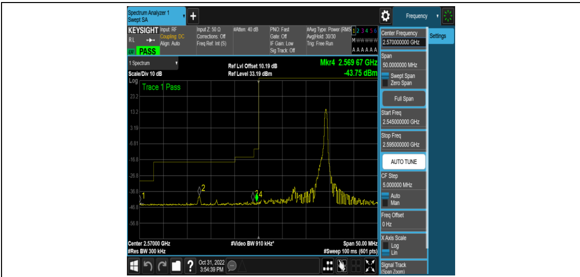
Band38-15MHz-QPSK-37825-75RB#0
