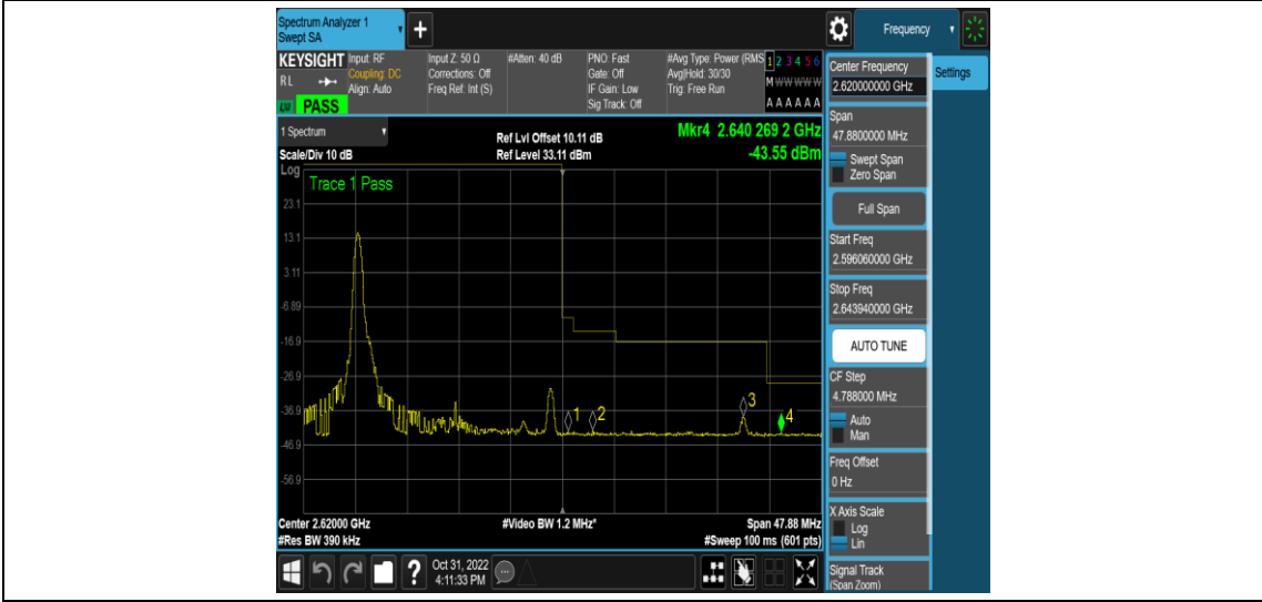
Band38-20MHz-16QAM-38150-1RB#99
