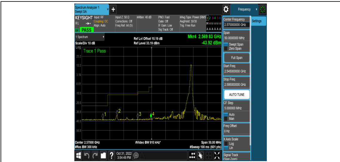
Band38-15MHz-16QAM-37825-75RB#0
