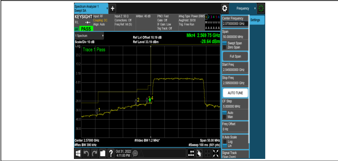
Band38-20MHz-16QAM-38150-1RB#0
