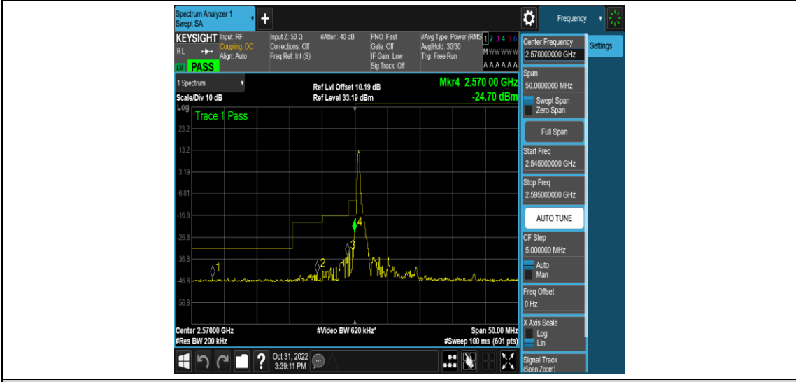
Band38-10MHz-16QAM-37800-1RB#49
