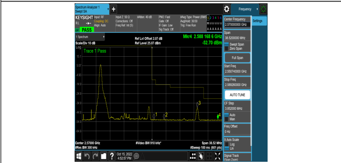
Band7-15MHz-QPSK-21375-1RB#74
