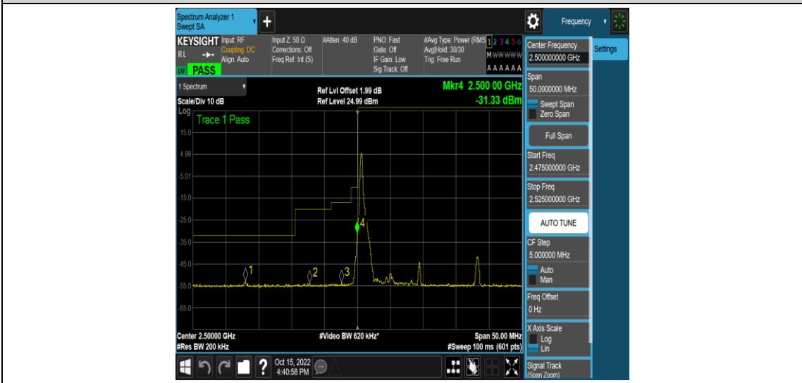
Band7-10MHz-16QAM-20800-1RB#49
