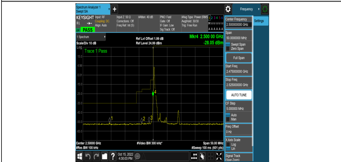
Band7-5MHz-16QAM-20775-1RB#24
