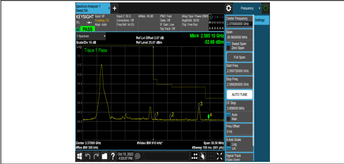
Band7-15MHz-16QAM-21375-1RB#74
