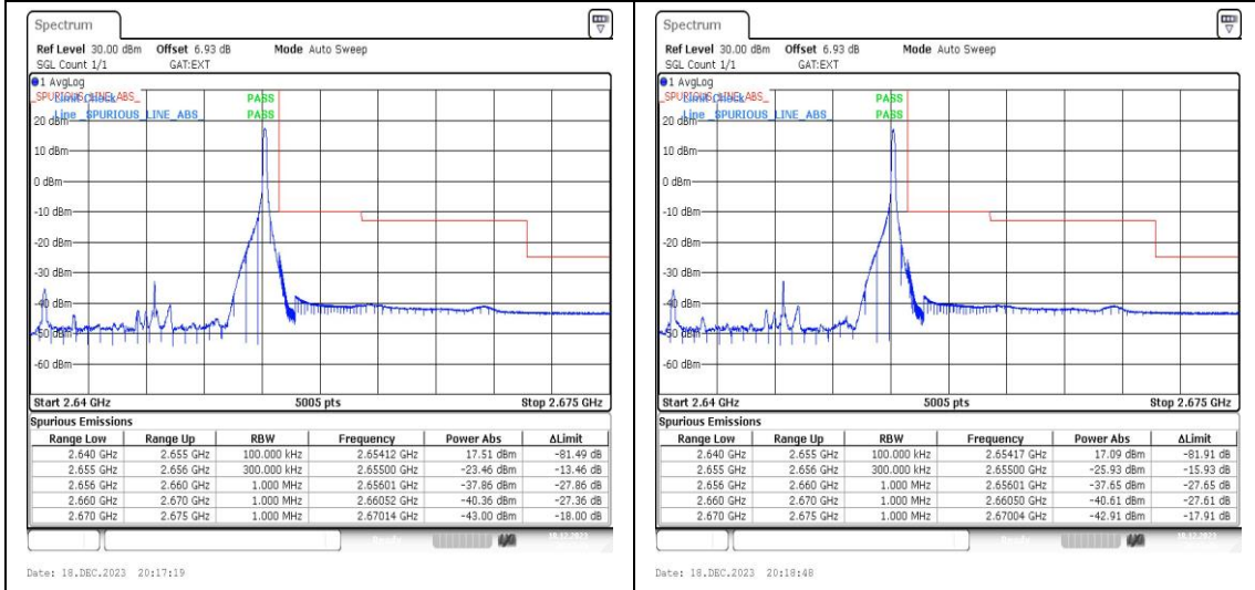
Band41_15MHz_QPSK_41165_1RB#74
