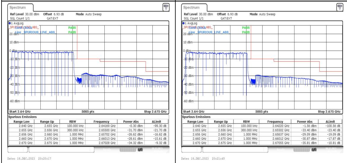
Band41_15MHz_QPSK_41165_75RB#0
