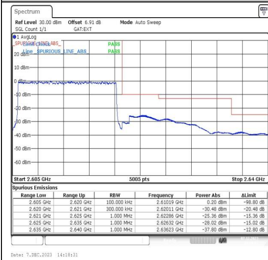
Band38_15MHz_QPSK_38175_75RB#0
