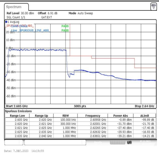
Band38_15MHz_16QAM_38175_75RB#0
