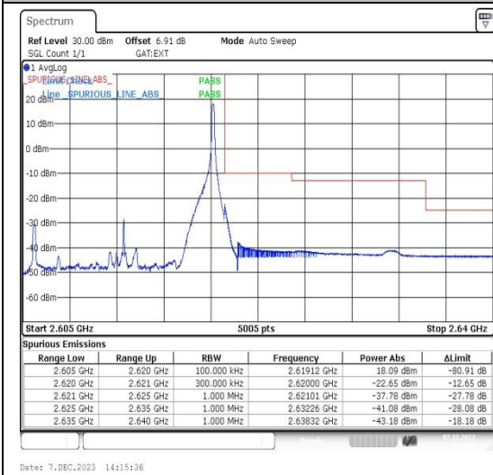
Band38_15MHz_QPSK_38175_1RB#74
