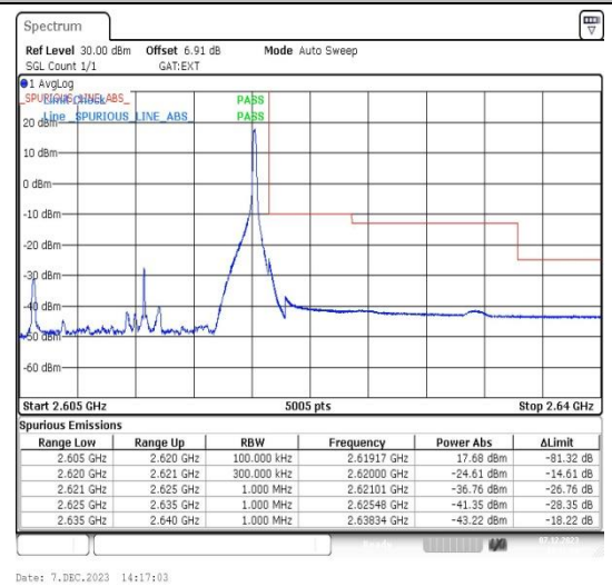
Band38_15MHz_16QAM_38175_1RB#74
