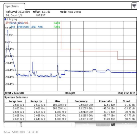
Band38_15MHz_16QAM_38175_1RB#0
