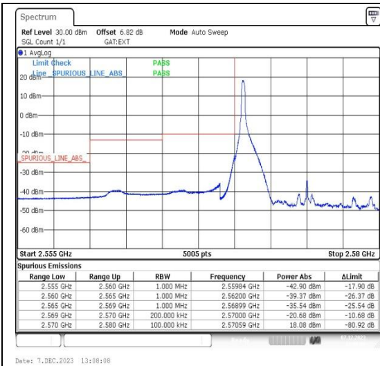
Band38_10MHz_QPSK_37800_1RB#0
