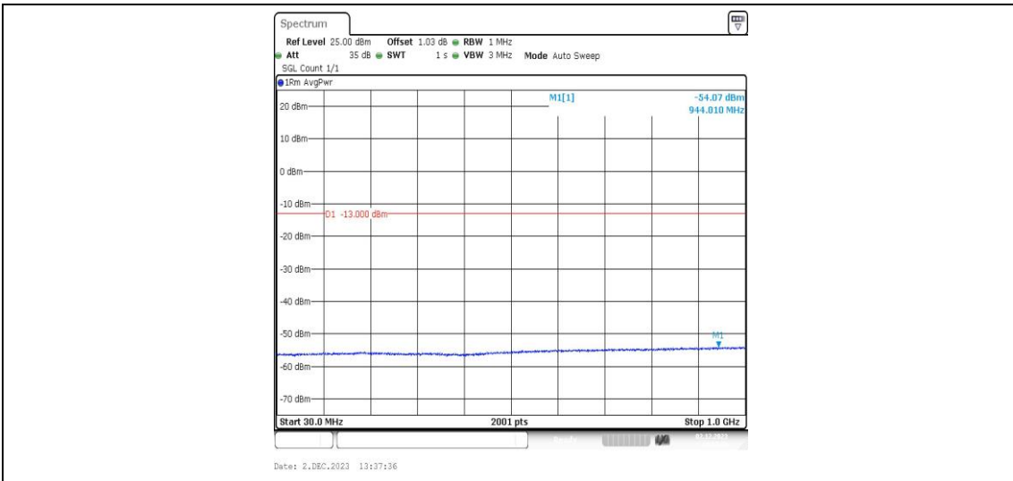
Band2-9400-4-30~1000MHz-PASS
