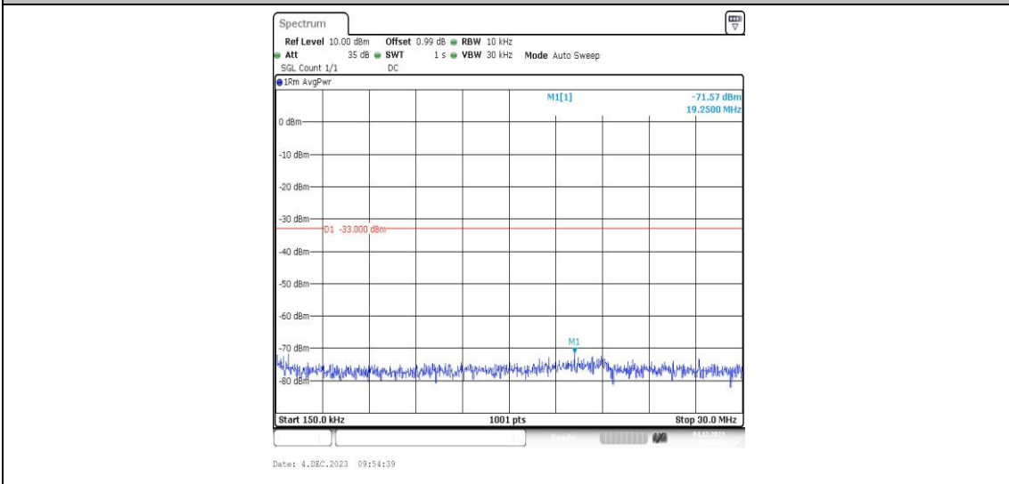
Band4-1312-4-0.15~30MHz-PASS
