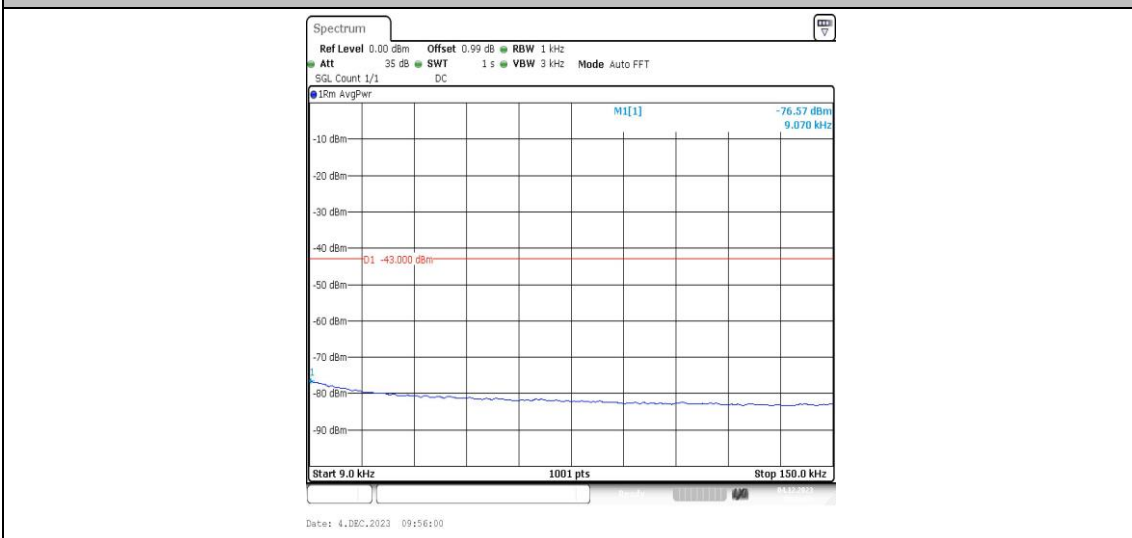
Band4-1513-4-0.009~0.15MHz-PASS
