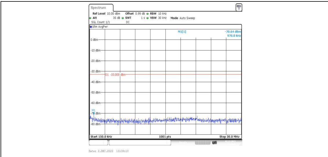
Band2-9538-4-0.15~30MHz-PASS
