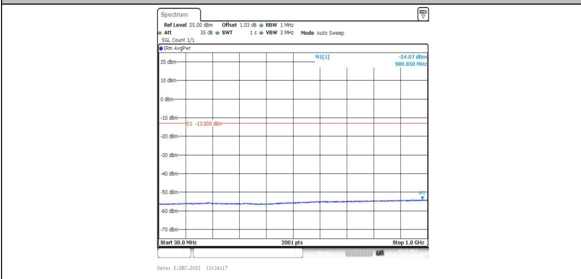
Band2-9262-3-30~1000MHz-PASS
