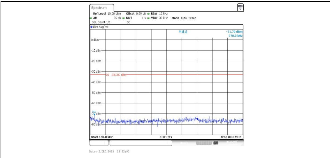
Band2-9538-2-0.15~30MHz-PASS
