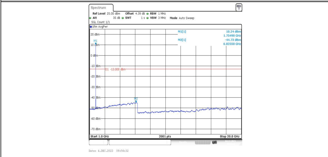
Band4-1513-4-1000~20000MHz-PASS
