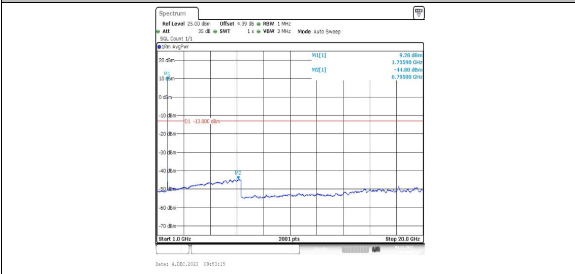
Band4-1413-3-1000~20000MHz-PASS
