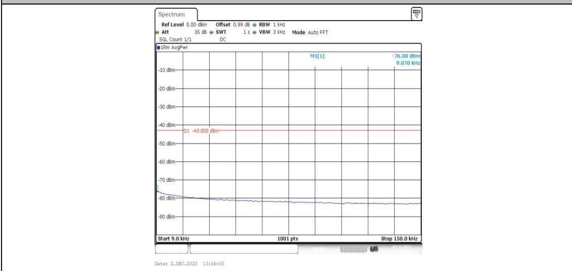
Band2-9538-4-0.009~0.15MHz-PASS
