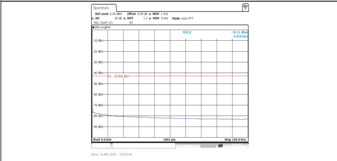
Band4-1413-3-0.009~0.15MHz-PASS
