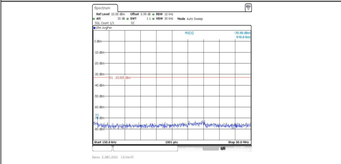
Band2-9262-3-0.15~30MHz-PASS
