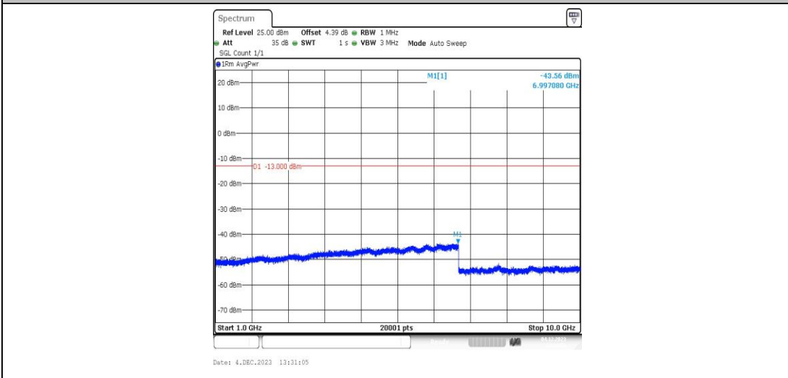
Band5-4182-2-1000~10000MHz-PASS
