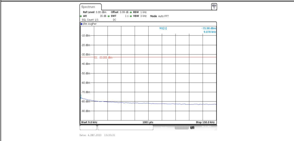
Band5-4182-2-0.009~0.15MHz-PASS
