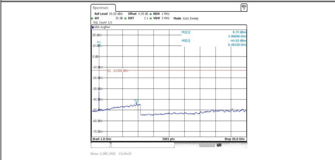
Band2-9538-4-1000~20000MHz-PASS
