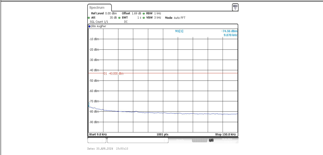
Band4-1413-1-0.009~0.15MHz-PASS
