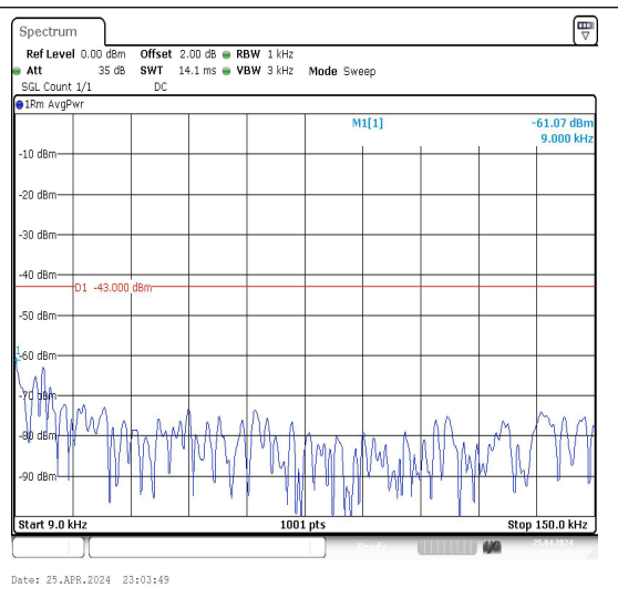
Band66_10MHz_16QAM_132022_1RB#0_0.009~0.15_0.009~0.15
