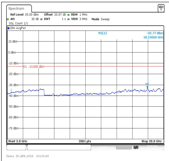
Band66_10MHz_QPSK_132022_1RB#0_3000~2000_3000~20000
