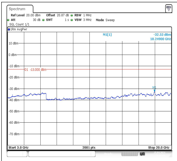
Band66_3MHz_QPSK_132322_1RB#0_3000~2000_000_3000~20000
