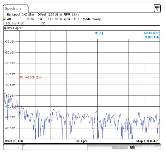
Band66_3MHz_16QAM_132322_1RB#0_0.009~0.000_3000~20000
