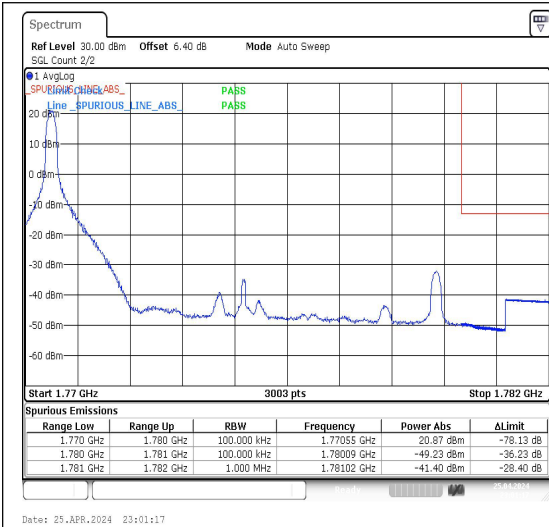
Band66_10MHz_QPSK_132622_1RB#0
