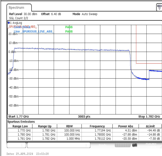
Band66_10MHz_QPSK_132622_50RB#0
