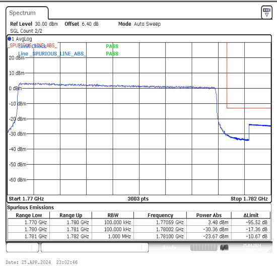
Band66_10MHz_16QAM_132622_50RB#0
