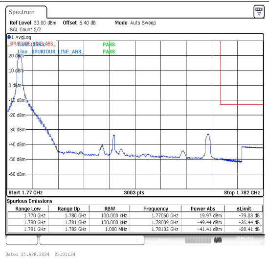
Band66_10MHz_16QAM_132622_1RB#0
