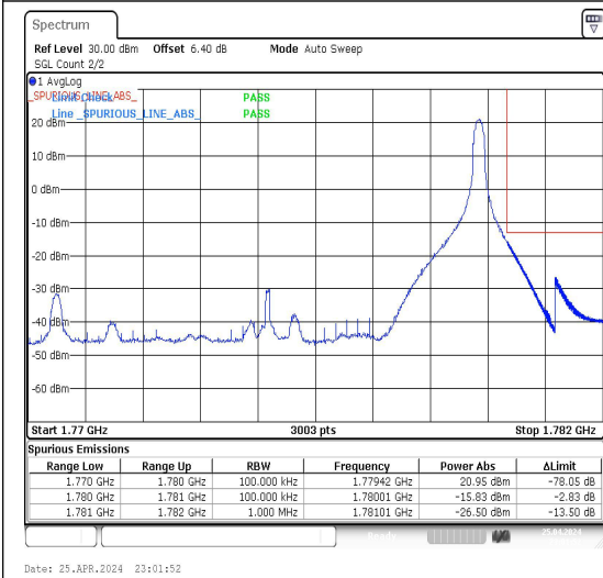
Band66_10MHz_QPSK_132622_1RB#49
