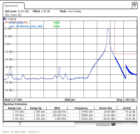
Band66_10MHz_16QAM_132622_1RB#49
