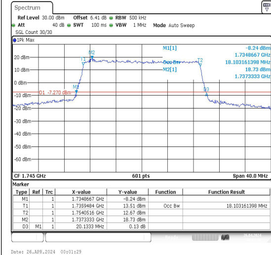
Band66-20MHz-QPSK-132322-100RB#0-PASS
