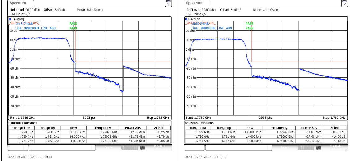
Band66_1.4MHz_QPSK_132665_6RB#0 Band66_1.4MHz_16QAM_132665_6RB#0
