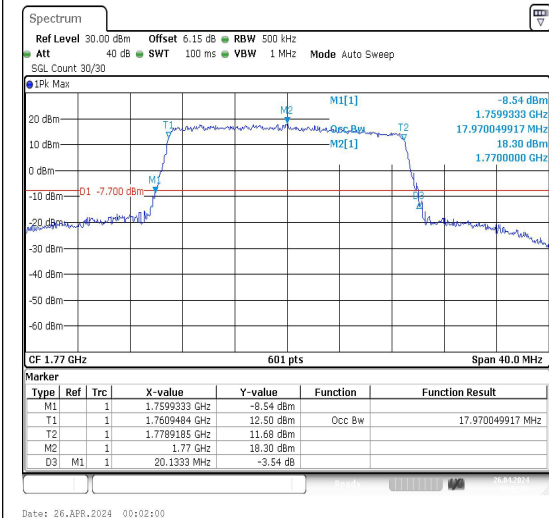
Band66-20MHz-QPSK-132572-100RB#0-PASS
