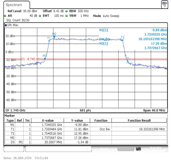
Band66-20MHz-16QAM-132322-100RB#0-PASS
