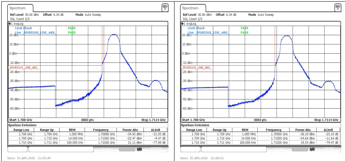
Band66_1.4MHz_QPSK_131979_1RB#0 Band66_1.4MHz_16QAM_131979_1RB#0
