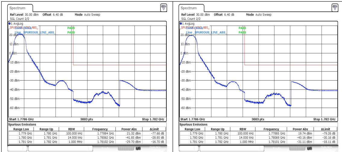
Band66_1.4MHz_QPSK_132665_1RB#0 Band66_1.4MHz_16QAM_132665_1RB#0
