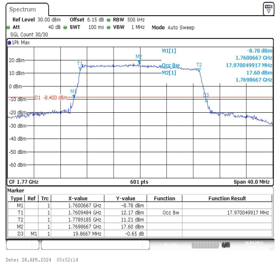
Band66-20MHz-16QAM-132572-100RB#0-PASS
