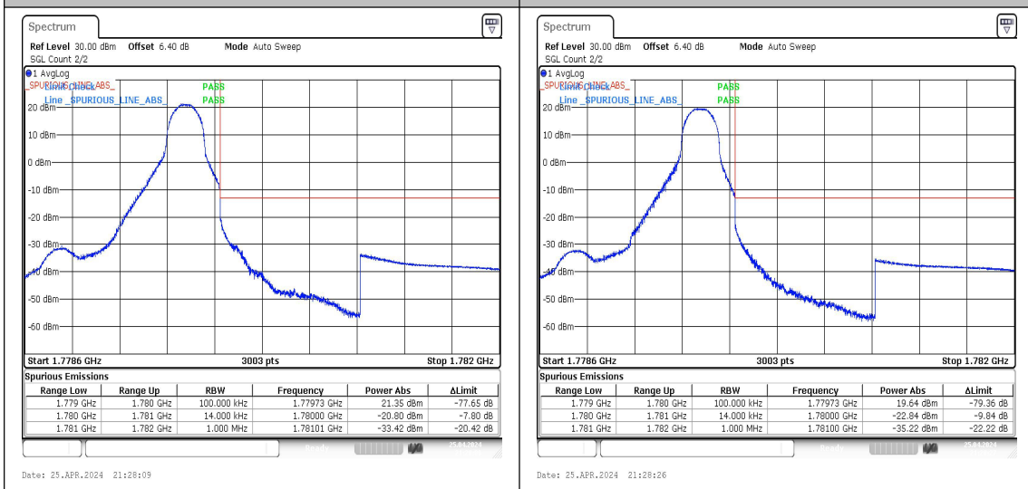
Band66_1.4MHz_QPSK_132665_1RB#5 Band66_1.4MHz_16QAM_132665_1RB#5
