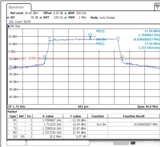
Band66-20MHz-QPSK-132072-100RB#0-PASS
