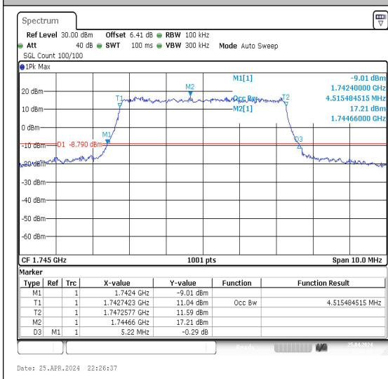
Band66-5MHz-QPSK-132322-25RB#0-PASS
