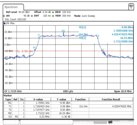
Band66-5MHz-16QAM-131997-25RB#0-PASS
