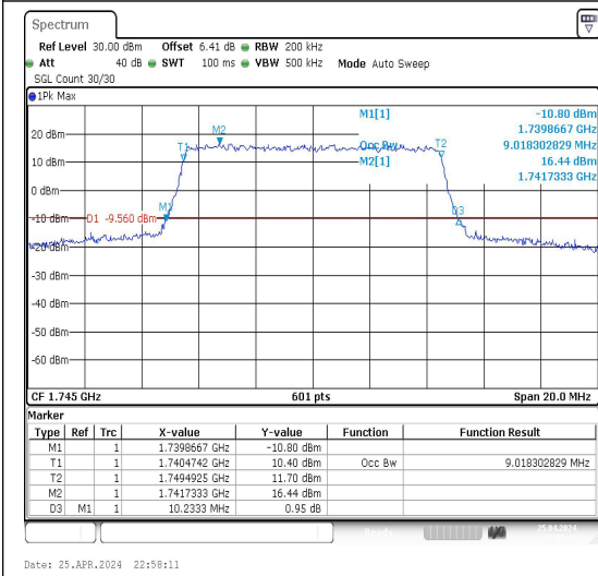
Band66-10MHz-QPSK-132322-50RB#0-PASS
