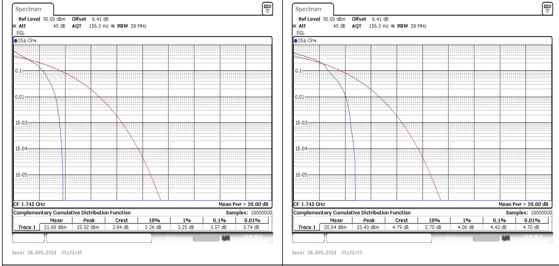
Band66-20MHz-QPSK-132322-1RB#0-PASS Band66-20MHz-16QAM-132322-1RB#0-PASS
