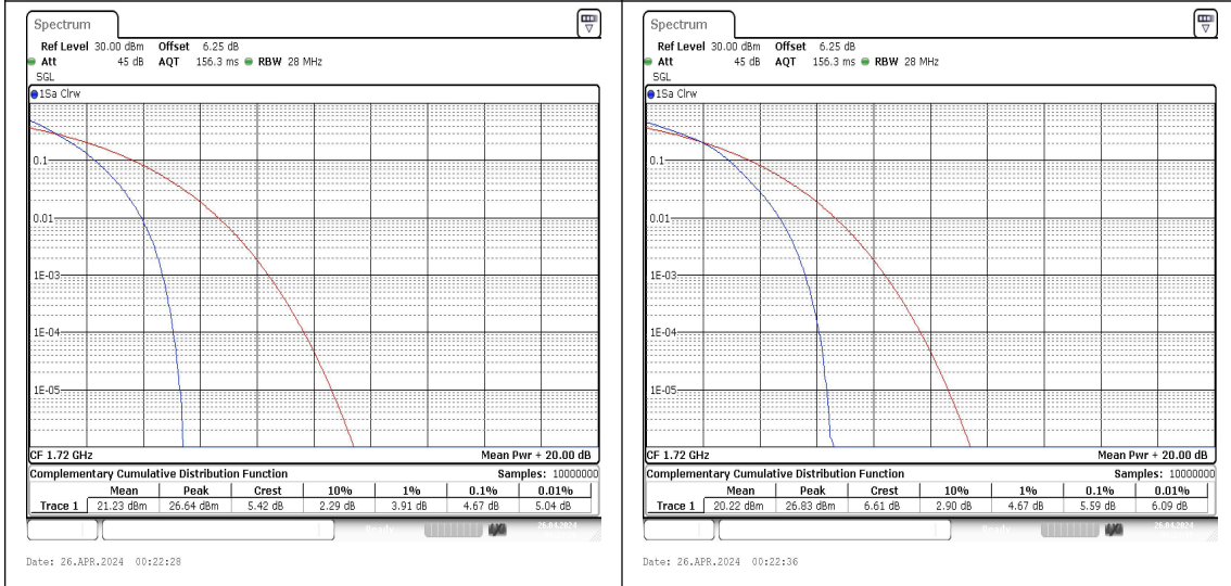
Band66-20MHz-QPSK-132072-100RB#0-PASS Band66-20MHz-16QAM-132072-100RB#0-PASS
