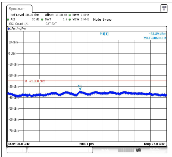
Band41_10MHz_QPSK_41190_1RB#0_20000~27000
