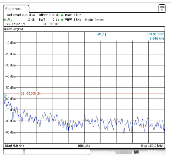
Band41_10MHz_16QAM_41190_1RB#0_0.009~0.15
