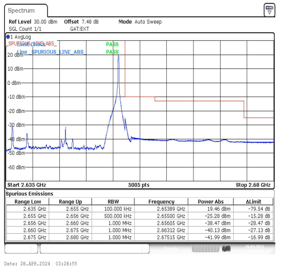
Band41_20MHz_16QAM_41140_1RB#99
