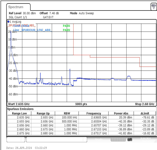
Band41_20MHz_QPSK_41140_1RB#0
