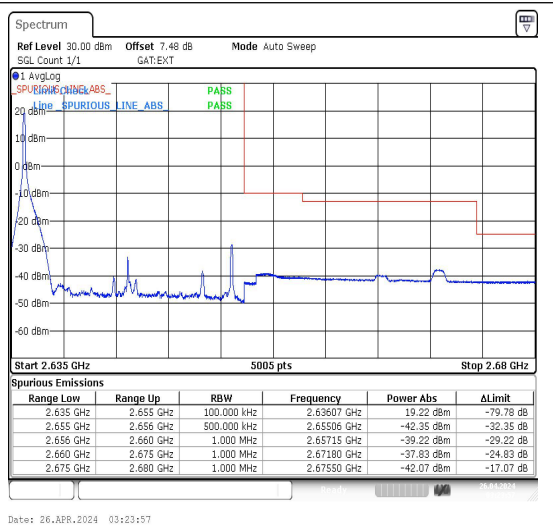
Band41_20MHz_16QAM_41140_1RB#0
