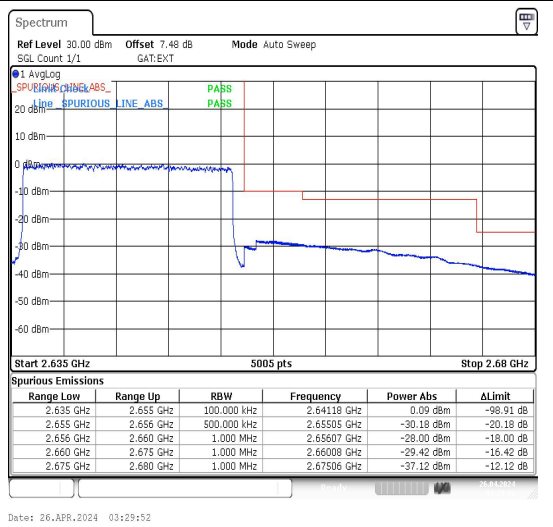
Band41_20MHz_16QAM_41140_100RB#0
