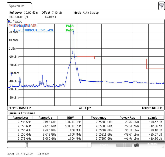
Band41_20MHz_QPSK_41140_1RB#99
