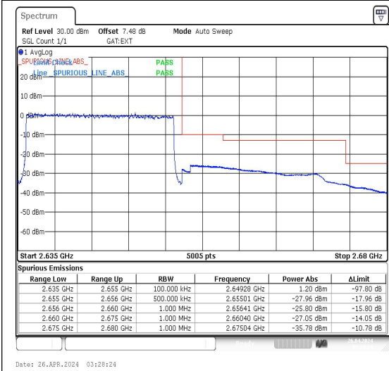
Band41_20MHz_QPSK_41140_100RB#0
