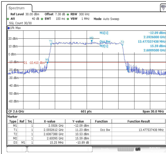
41(2555-2655)-15MHz-QPSK-40690-75RB#0-PA SS
