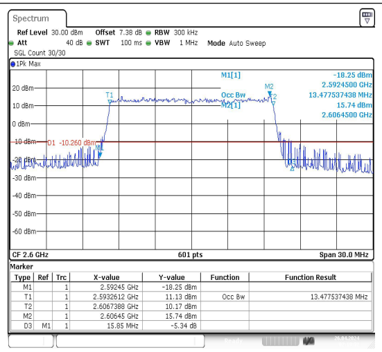
41(2555-2655)-15MHz-16QAM-40690-75RB#0-PA SS
