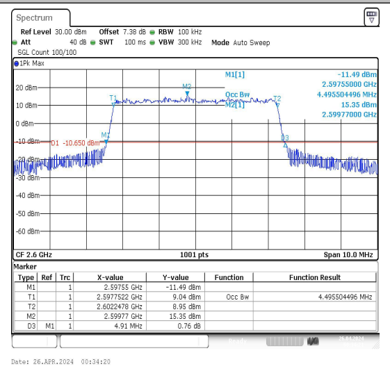
41(2555-2655)-5MHz-16QAM-40690-25RB#0-PAS S
