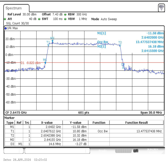
41(2555-2655)-15MHz-16QAM-41165-75RB#0-PA SS
