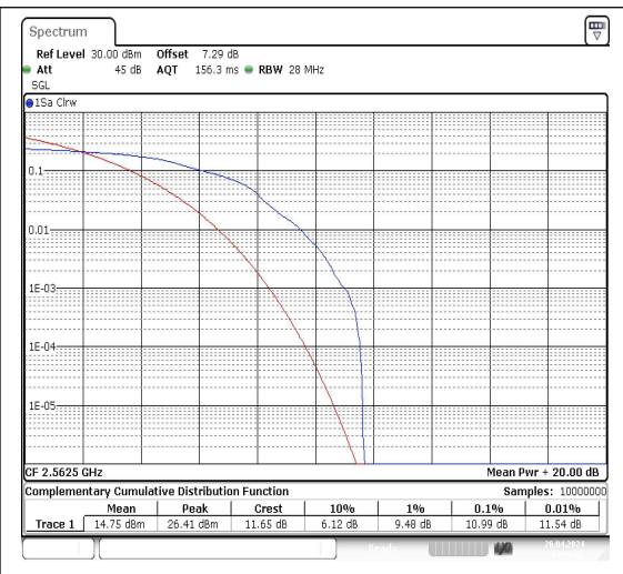
41(2555-2655)-15MHz-QPSK-40315-1RB#0-PAS S
