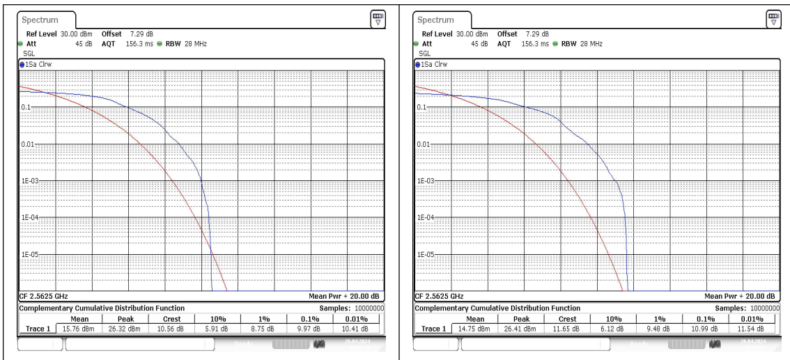
41(2555-2655)-15MHz-QPSK-40315-1RB#0-PAS S
