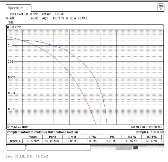
41(2555-2655)-15MHz-QPSK-40315-75RB#0-PA SS
