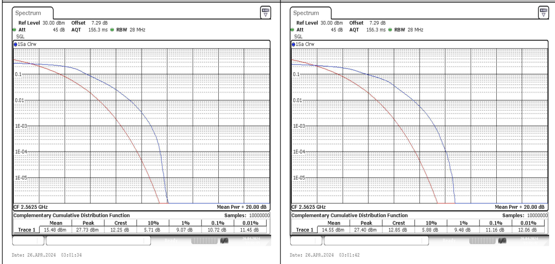
41(2555-2655)-15MHz-QPSK-40315-75RB#0-PA SS
