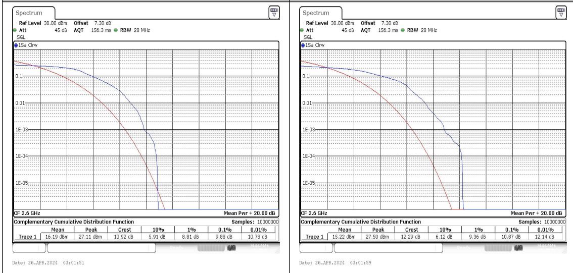
41(2555-2655)-15MHz-QPSK-40315-1RB#0-PAS S
