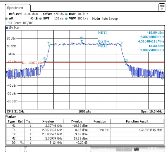
40(2305-2315)-5MHz-16QAM-38750-25RB#0-PAS
