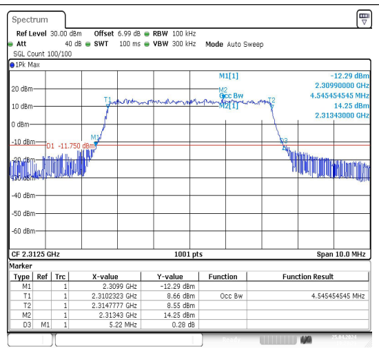
40(2305-2315)-5MHz-16QAM-38775-25RB#0-PAS S
