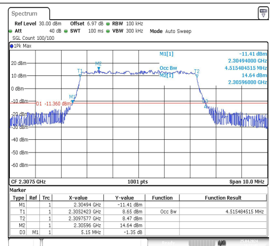
40(2305-2315)-5MHz-16QAM-38725-25RB#0-PAS
