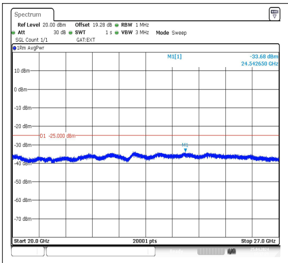
Band38_20MHz_QPSK_37850_1RB#0_20000~27000
