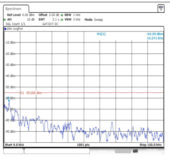
Band38_20MHz_16QAM_37850_1RB#0_0.009~0.15
