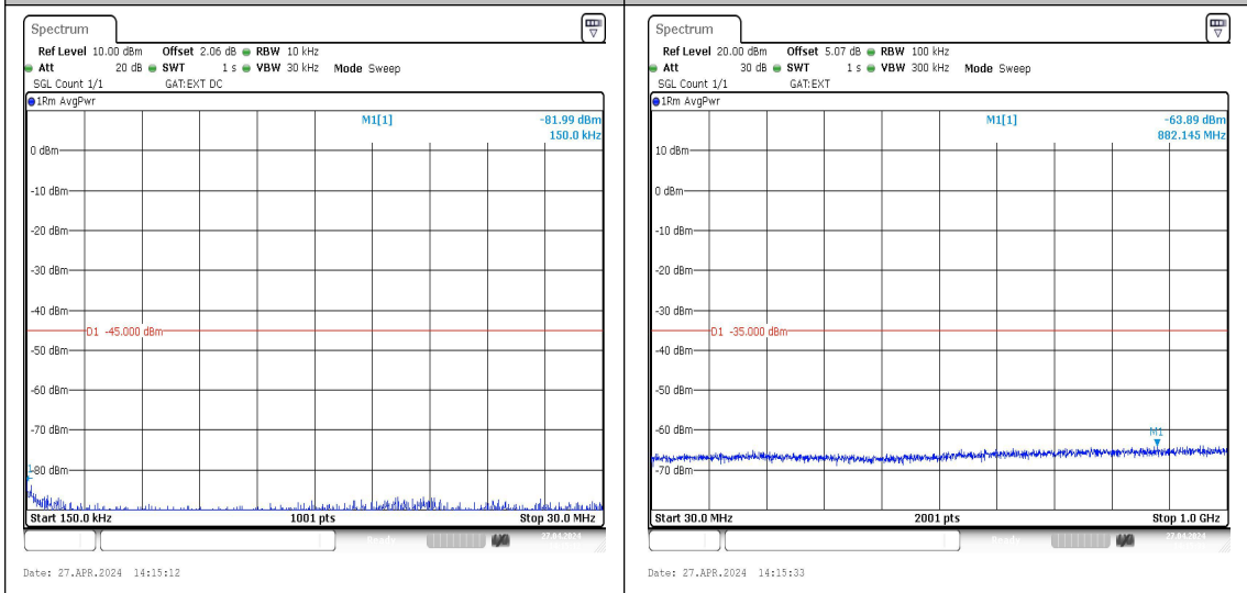
Date: 27.APR.2024 14:15:12 | Date: 27.APR.2024 14:15:33 Band38_15MHz_16QAM_38175_1RB#0_0.15~30 | Band38_15MHz_16QAM_38175_1RB#0_30~1000
