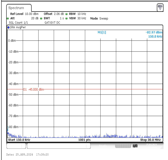
Band38_20MHz_16QAM_37850_1RB#0_0.15~30
