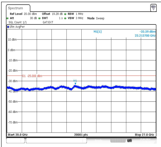
Band38_10MHz_QPSK_38200_1RB#0_20000~27000_20000~27000
