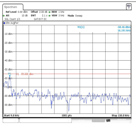
Band38_10MHz_16QAM_38200_1RB#0_0.009~0.15_0.009~0.15
