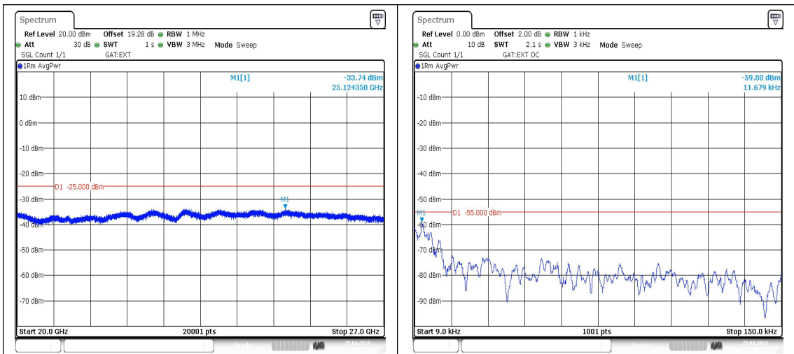
Band38_5MHz_QPSK_38225_1RB#0_20000~27000 000_20000~27000
