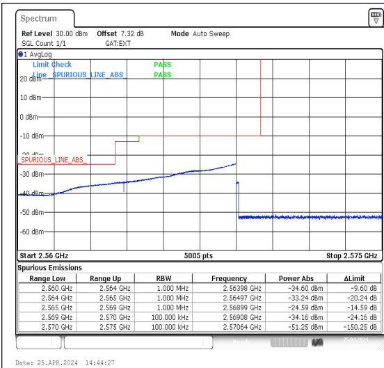
Band38_5MHz_QPSK_37775_25RB#0
