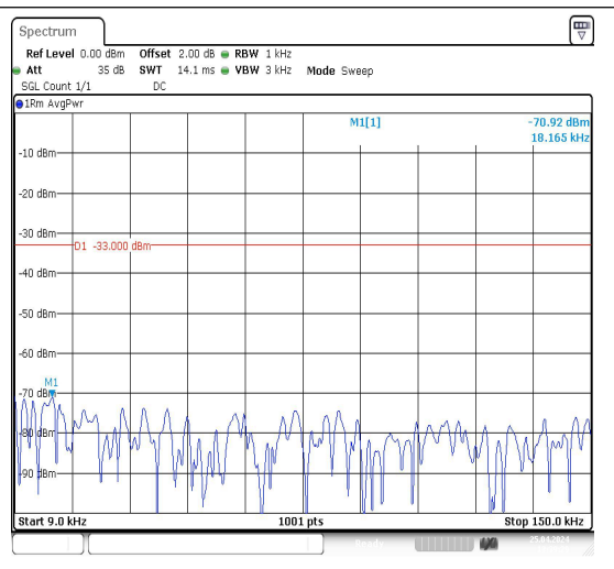
Band17_5MHz_16QAM_23825_1RB#0_0.009~0.15_5_0.009~0.15
