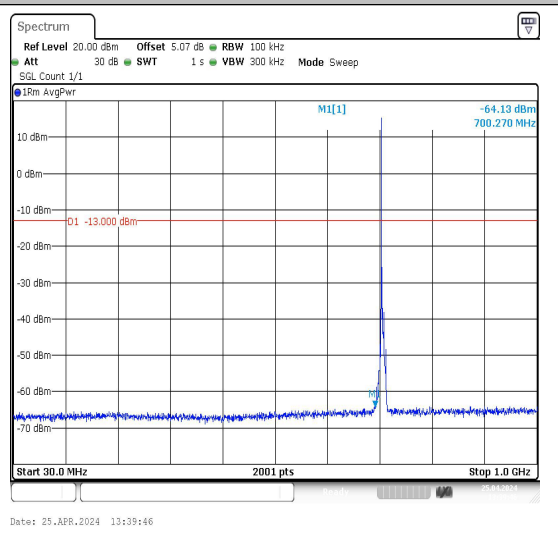
Band17_5MHz_16QAM_23825_1RB#0_30~1000_30~1000
