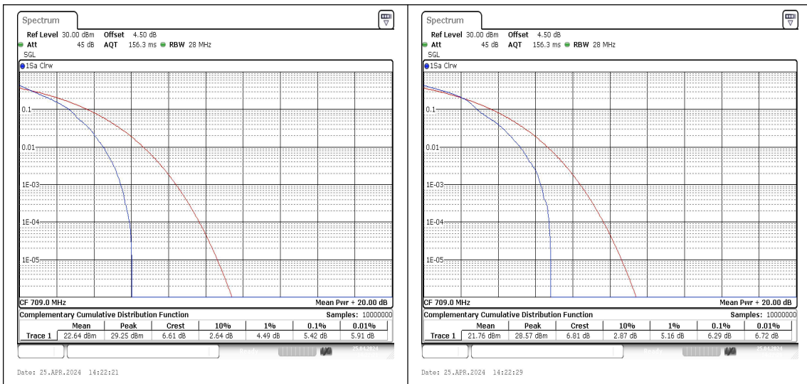
Band17-10MHz-QPSK-23780-1RB#0-PASS Band17-10MHz-16QAM-23780-1RB#0-PASS
