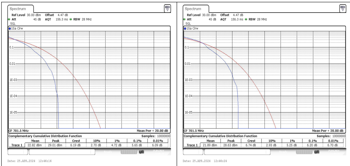
Band12-5MHz-QPSK-23035-1RB#0-PASS Band12-5MHz-16QAM-23035-1RB#0-PASS
