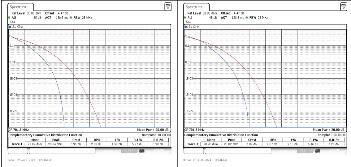
Band12-5MHz-QPSK-23035-25RB#0-PASS Band12-5MHz-16QAM-23035-25RB#0-PASS
