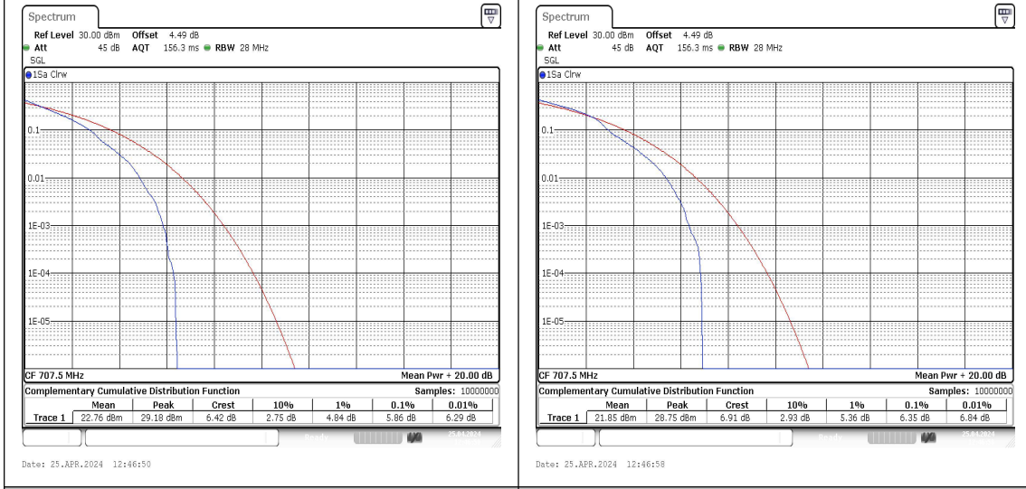
Band12-5MHz-QPSK-23095-1RB#0-PASS Band12-5MHz-16QAM-23095-1RB#0-PASS
